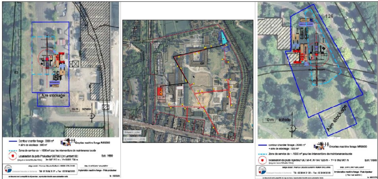
Illustration 6 – source CFG
